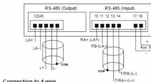
Connection to 4 wire
