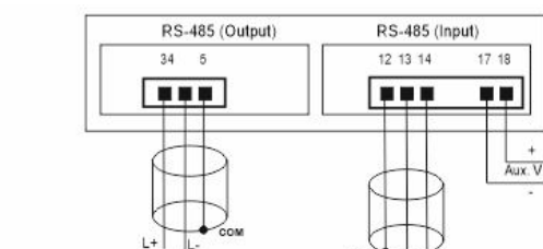
Connection to 2 wire
